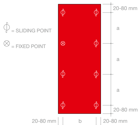
SINGLE SPAN PANEL
