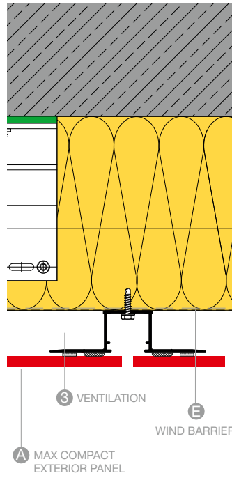
VERTICAL JOINT A107
