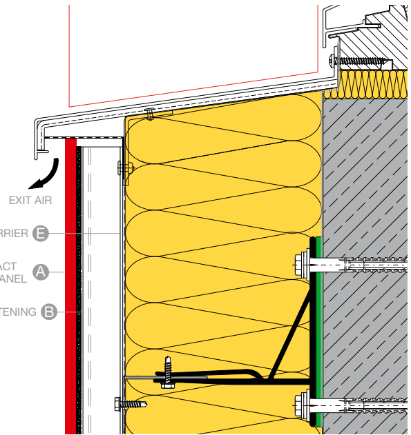
WINDOW SILL CONNECTION A102
